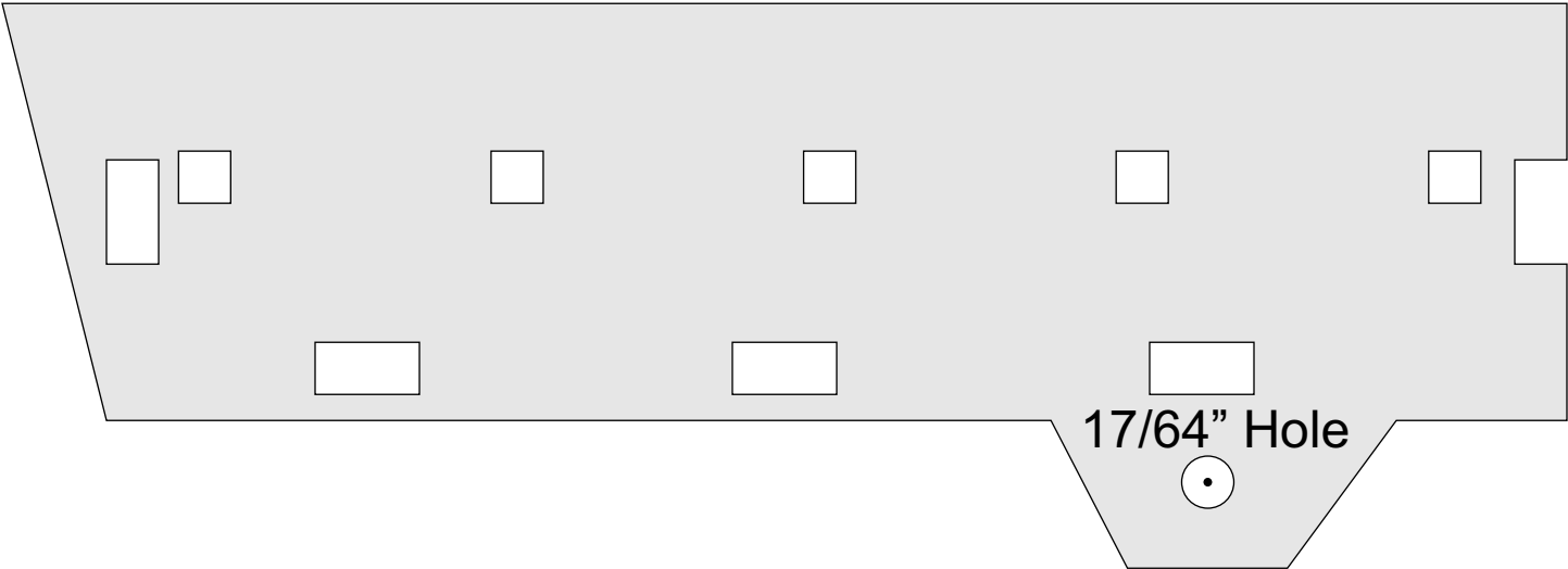
Wagon Slides Cut Two
