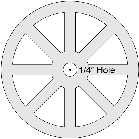
Front Wheels Cut Two
