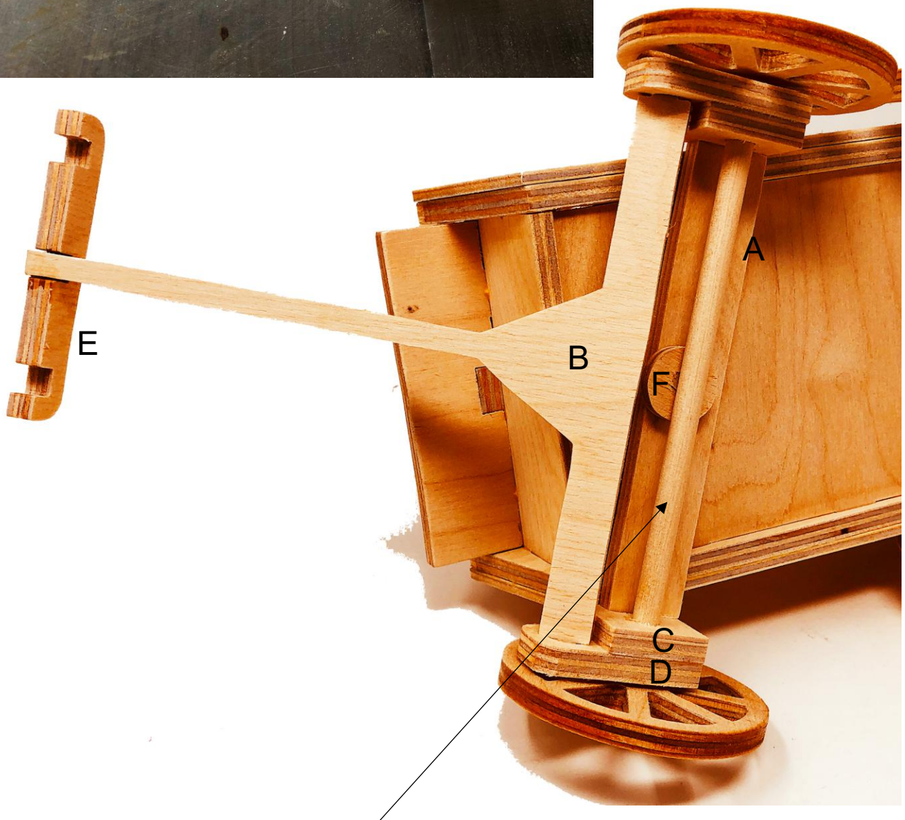
1/4" Diameter wooden dowel cut to fit.
