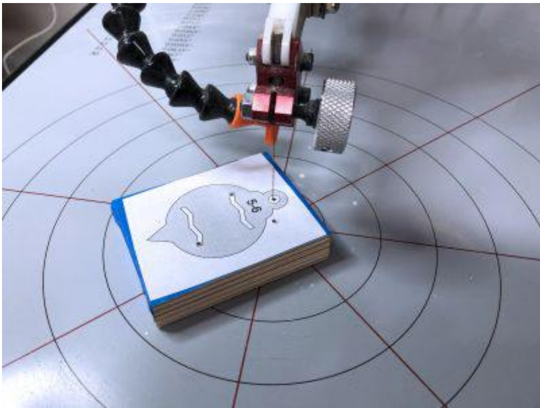
Stack cut
