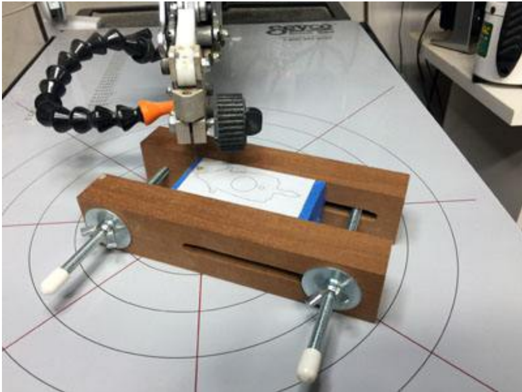
A compound cutting jig makes the process easier.
